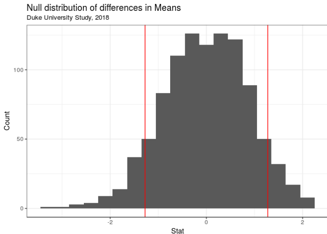
Figure 6: p\text{-value} = 0.132
