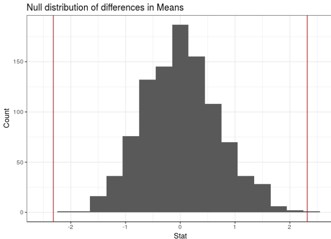
Figure 8: p\text{-value} = 0
